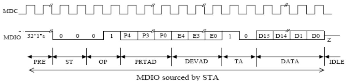
Figure 21 MDIO/MDC Timing Diagram during the Write/Address Operation
